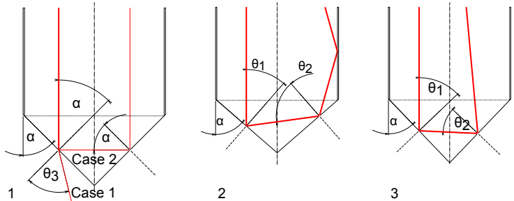
Fig. 1: (1) Tip-angle of 45 degrees, showing case 1 for transmission of light due to liquid and case 2 for total reflection due to gas at probe-tip; (2) maximum tip-angle (3) minimum tip-angle.
